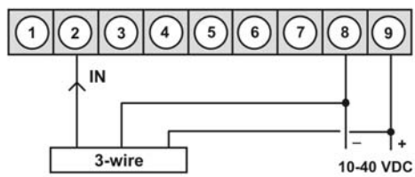
3-wire PNP
