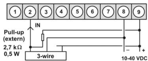
3-wire NPN
