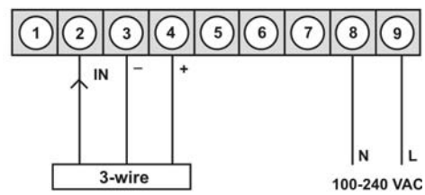
3-wire PNP
