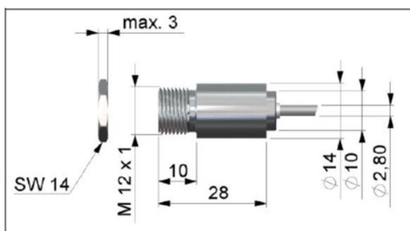
Sensing head
