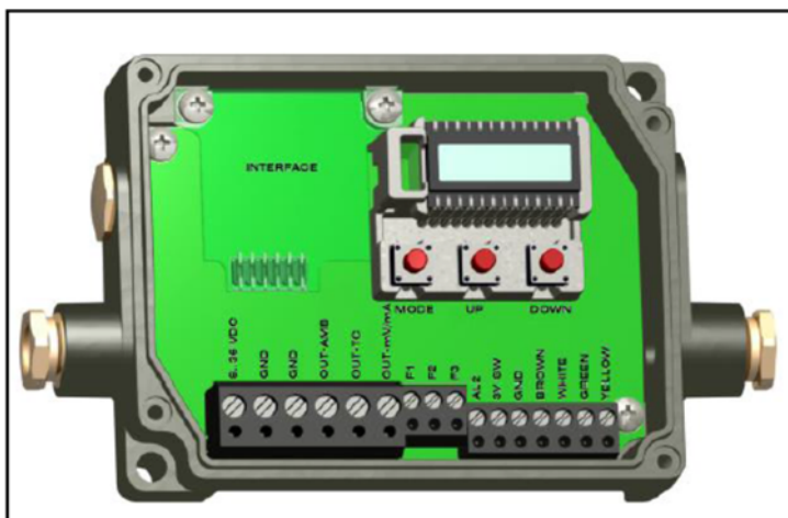
Opened electronic box with terminal connections
